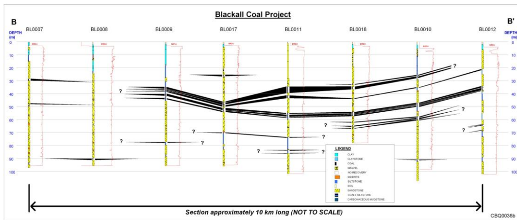
Figure 3: Blackall Coal Project Section B-B'
